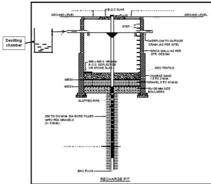
Figure 1: Schematic Diagram of Rain Water Harvesting Pit
