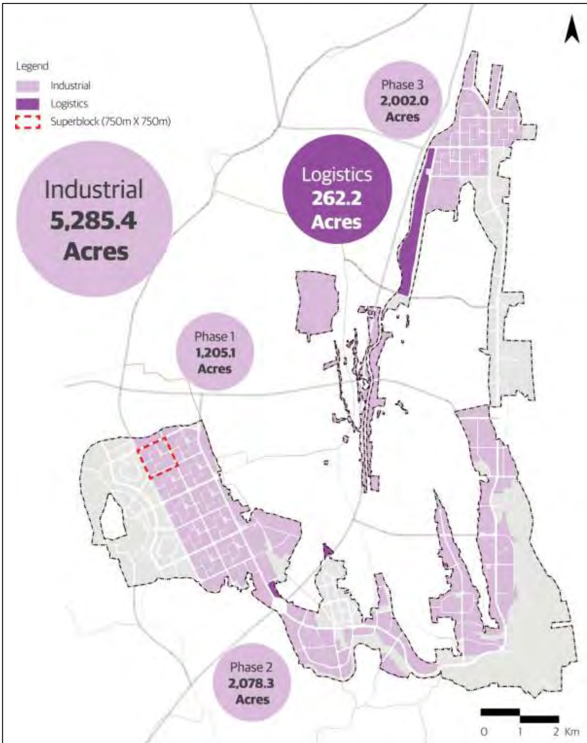
Figure 6-6 Industrial and Logistics Land Use
