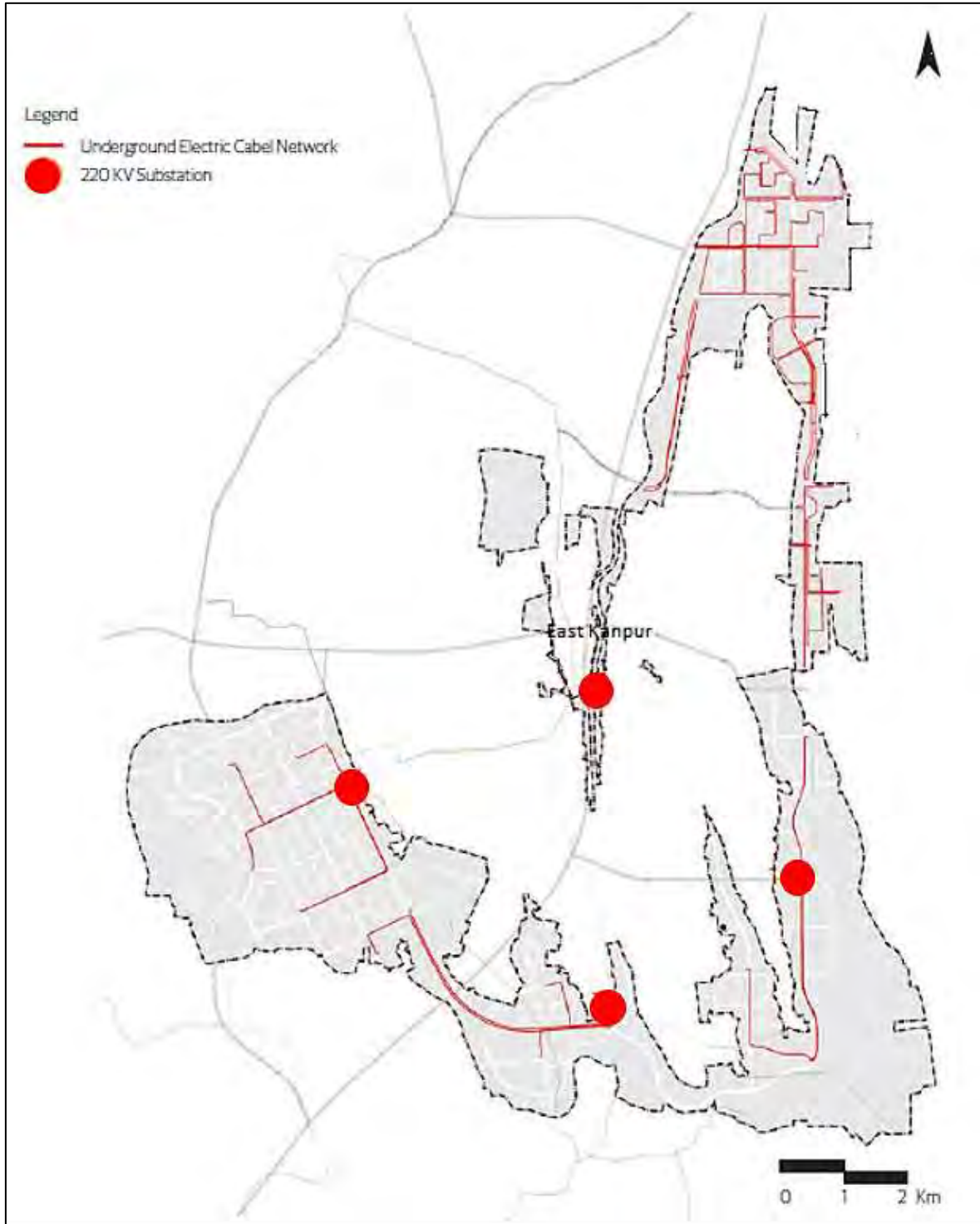
Figure 6-3: North Node Power Distribution Network
