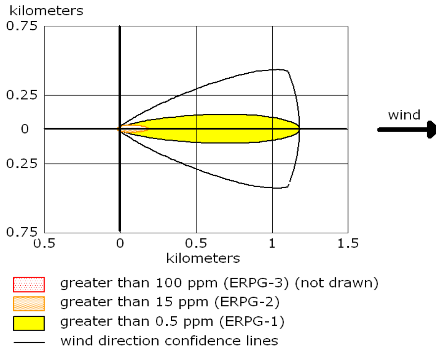
Figure 7.3 Acetic Anhydride Leak Toxic Impact
