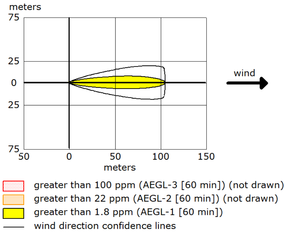
Figure 7.2: Hydrochloric Acid Tank leakage Toxic Impact
