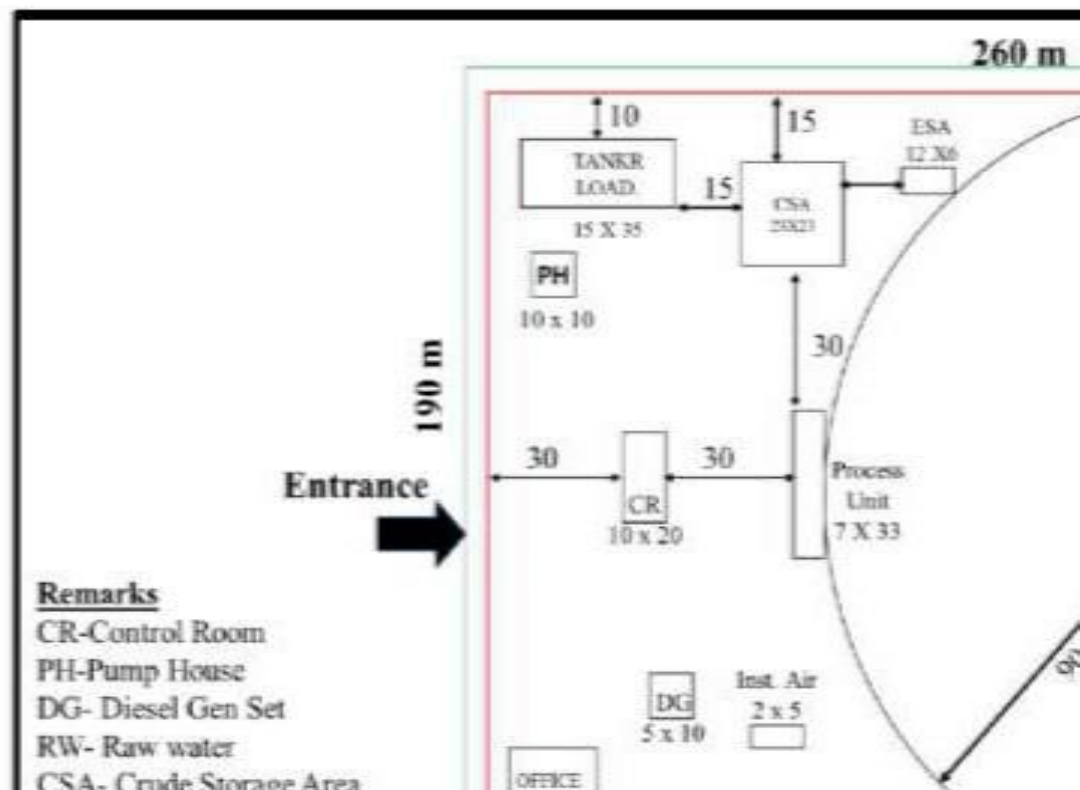
FIGURE 28 : EPS LAYOUT
