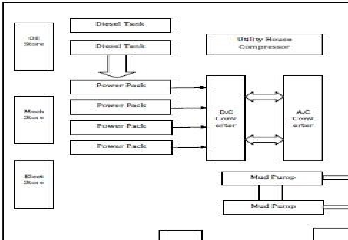
FIGURE 28 : EPS LAYOUT
