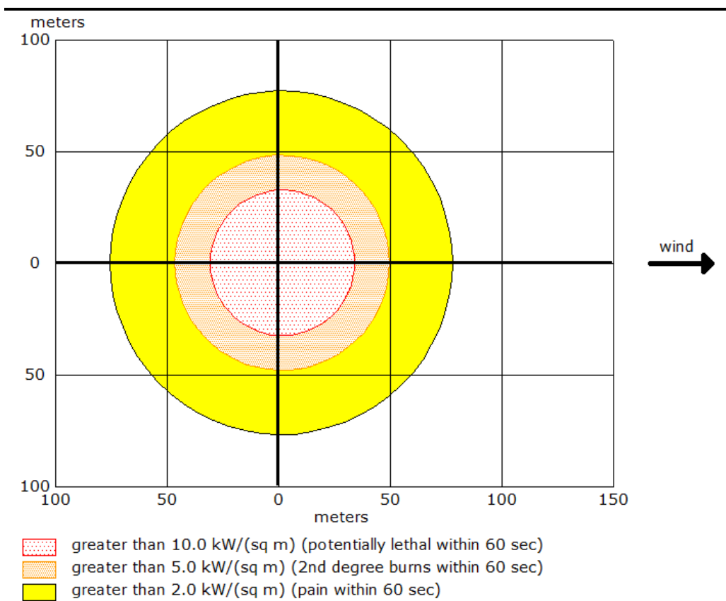
Figure 1.18 Threat Zone Plot – 250mm dia pipeline rupture
