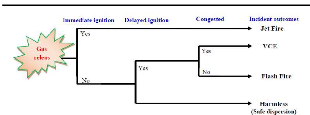
Figure 1.11 Natural Gas Release – Potential Consequences
