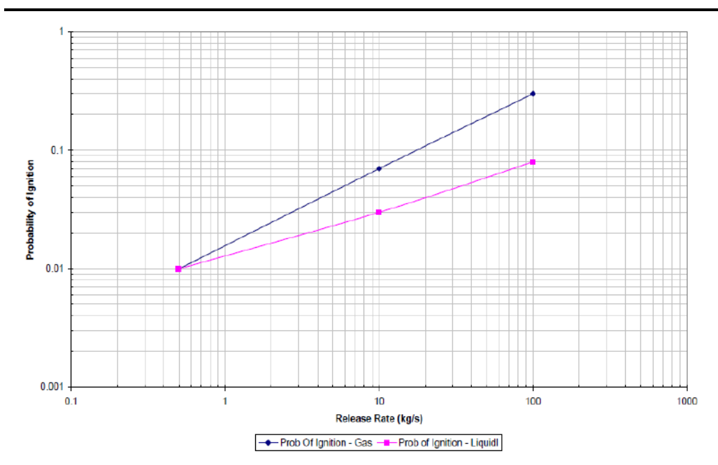
Figure 1.2 Ignition Probability Vs Release Rate
