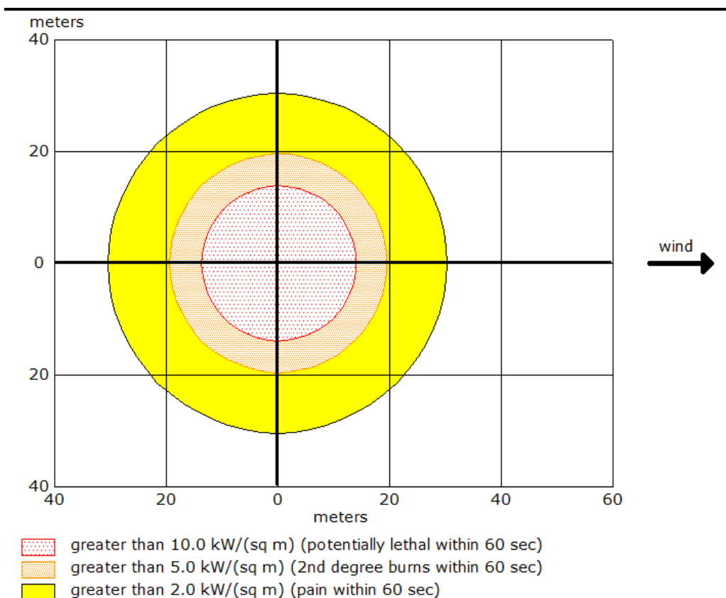
Figure 1.15 Threat Zone Plot –200mm dia pipeline leak (50mm dia)
