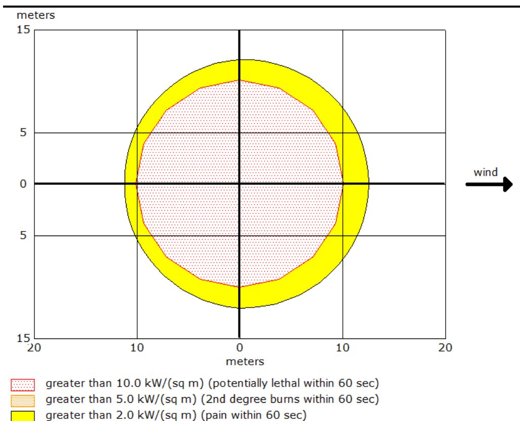
Figure 1.12 Threat Zone Plot – 50mm dia pipeline complete rupture
