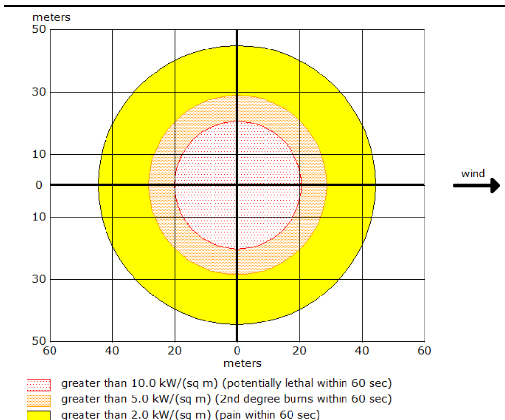
Figure 1.13 Threat Zone Plot - 300mm dia pipeline leak (75mm dia)
