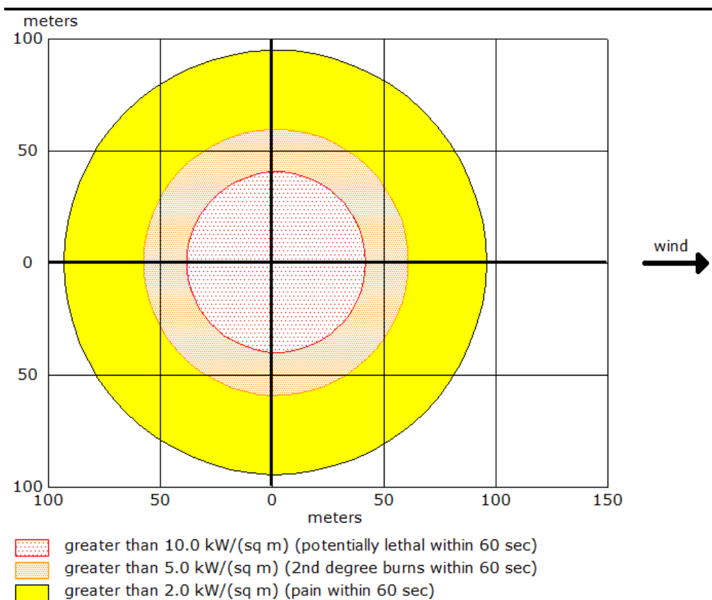
Figure 1.14 Threat Zone Plot – 300mm dia pipeline rupture
