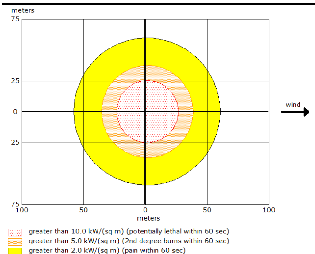
Figure 1.16 Threat Zone Plot -200mm dia pipeline rupture
