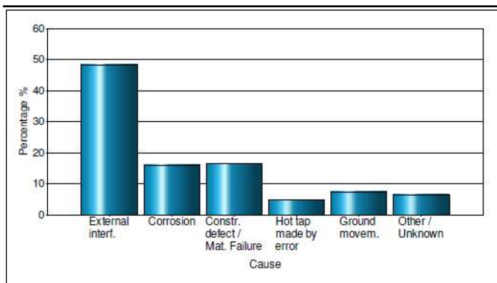
Figure 1.10 Gas Pipeline Failure – Distribution of Incident & Causes
