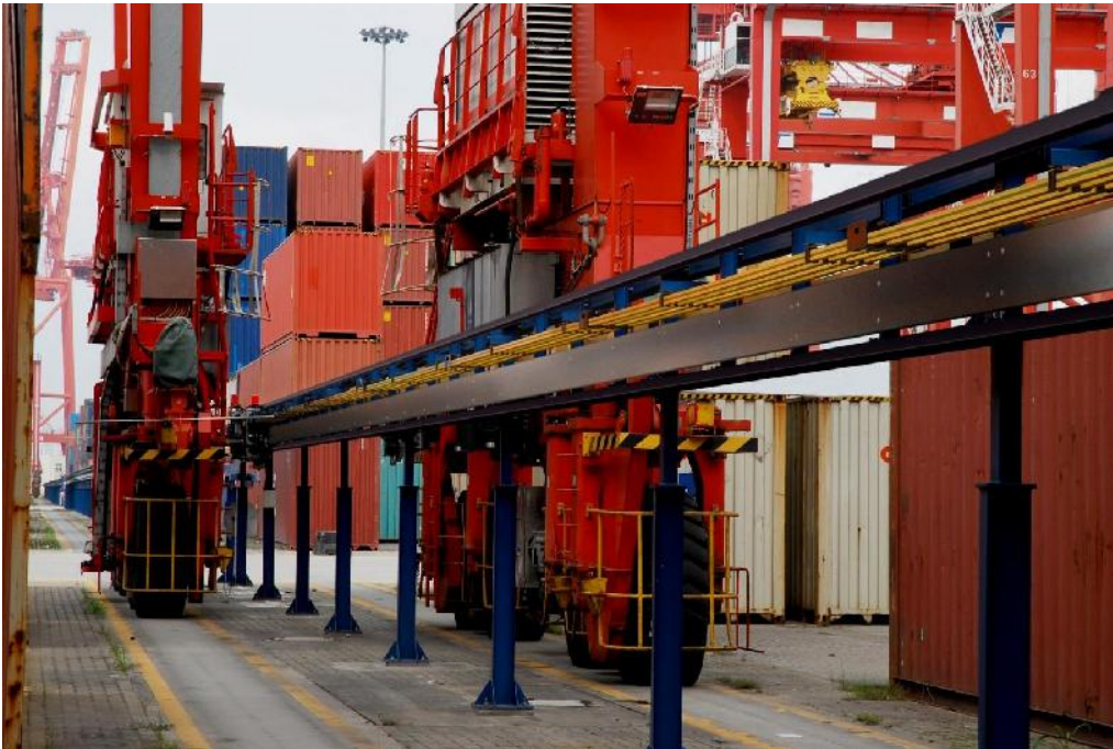
Figure 7.11 Typical Details of Electric Buss Bar Arrangement for E-RTG
