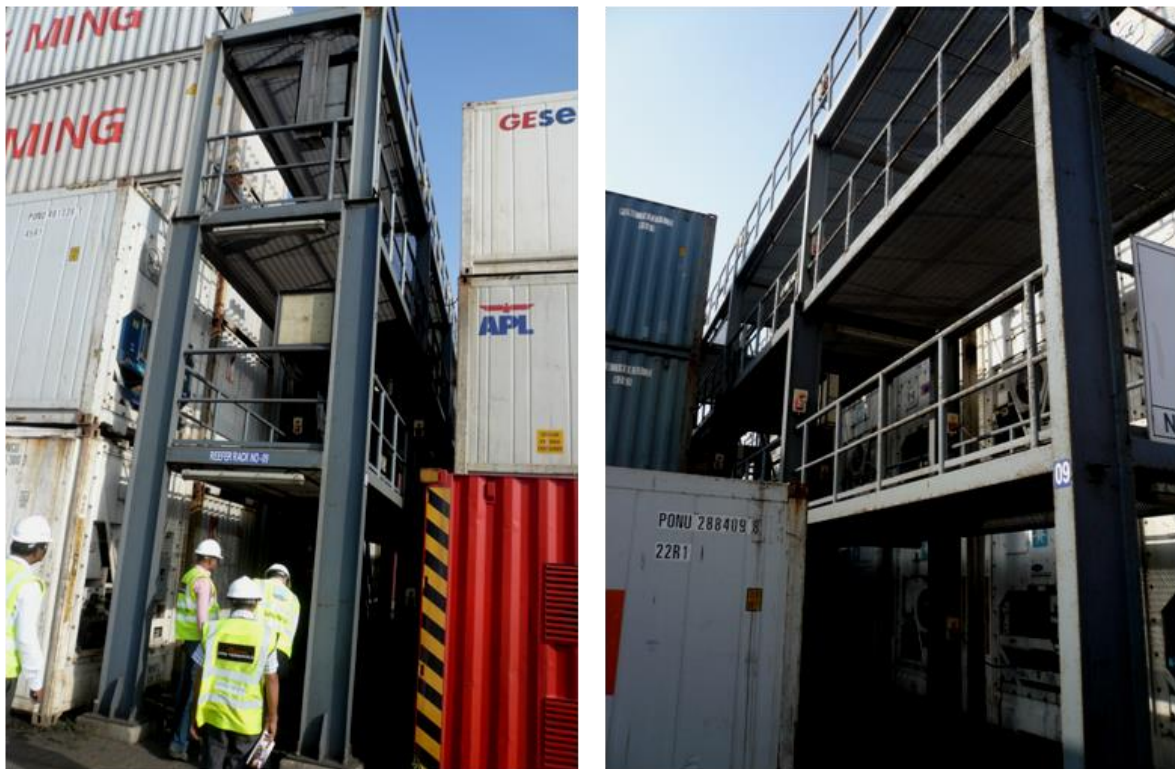
Figure 7.12 Typical Details of Reefer Stacks
